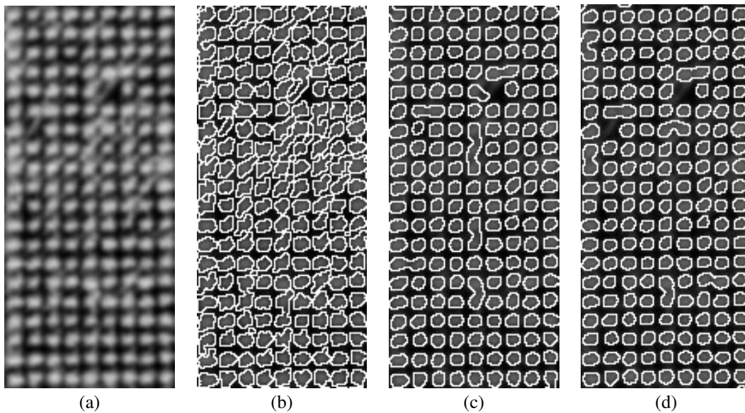
Figure 2: Experimental results: (a) an image of poplars ©IFN (0.86,0.06,0.43,0.2,3.5); (b) the best result with a CAC model (35000, 100, 500); (c) the best result with the HOAC ‘gas of circles’ model (1200, 20, 100, 82); (d) the best result with the phase field ‘gas of circles’ model (1200, 239, 22.5, 16.8, 150).
